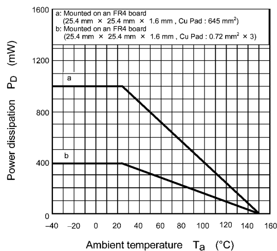
Fig. 8.13 P_D - T_a
