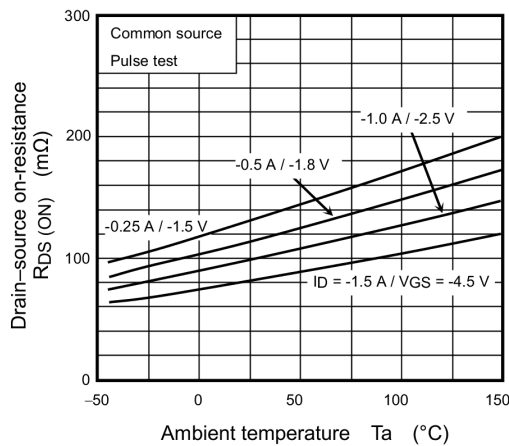
Fig. 8.5 R_{DS(ON)} - T_a
