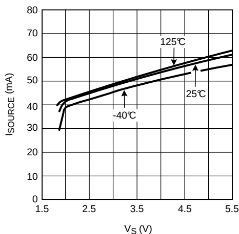
Figure 32. Sourcing Current vs. Supply Voltage
