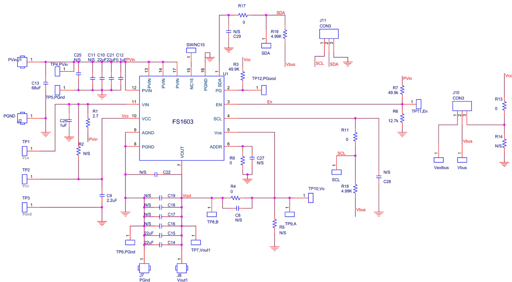
Figure 2 Schematic
