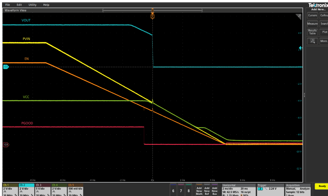
Figure 5 Shutdown with Enable de-assertion at 3A load (Ch1:PV IN , Ch2: V OUT , Ch3: PG, Ch4:V CC , Ch5: Enable)
