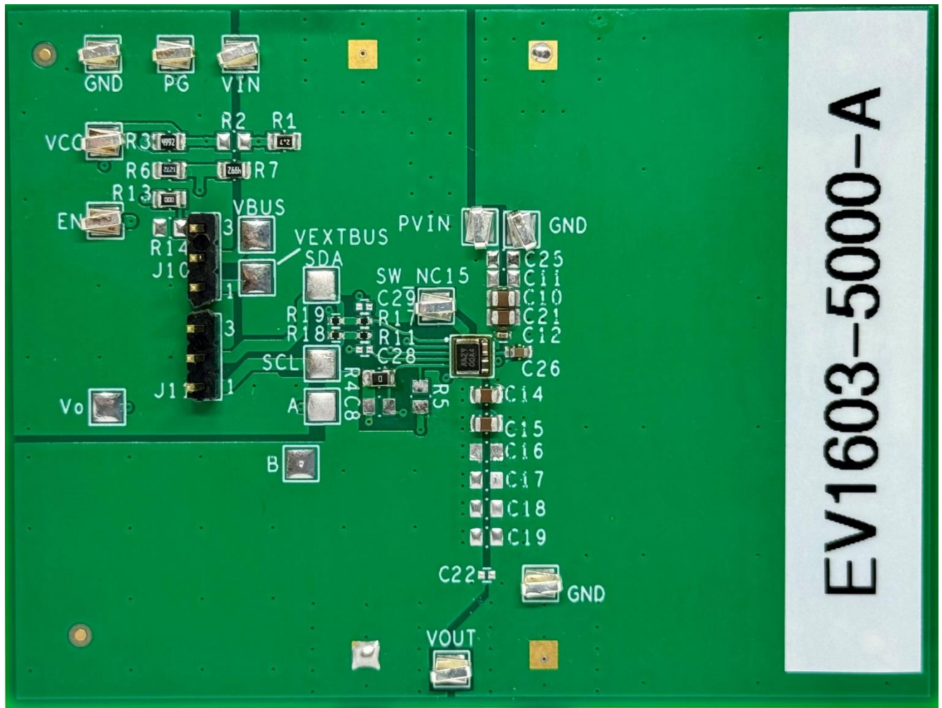
Figure 1 Board layout
