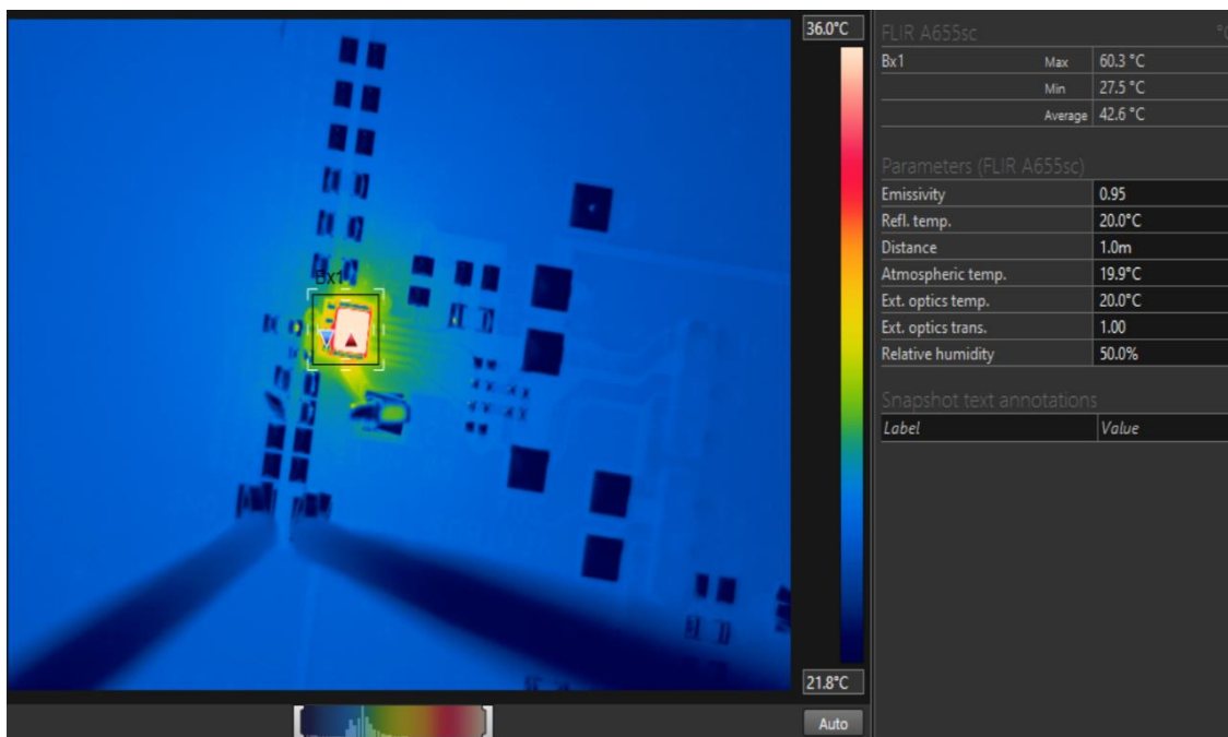
Figure 18 Thermal image( P_{VIN}=12V , I_{OUT}=3A ) – maximum temperature rise = 37^{\circ}C
