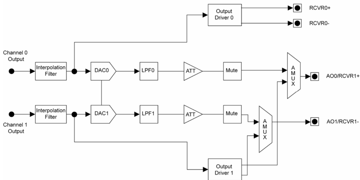
Figure 13: Output Stage
