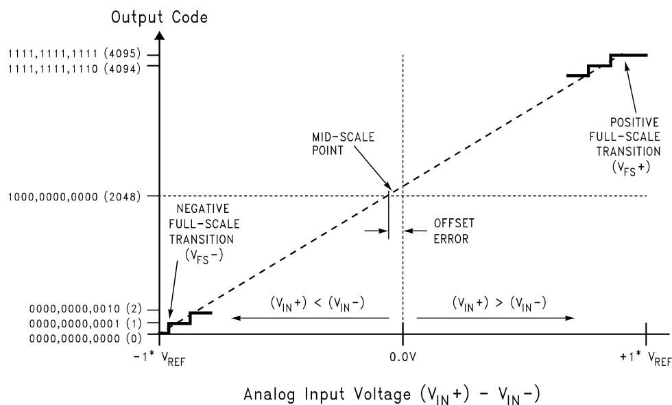
Figure 2. Transfer Characteristic
