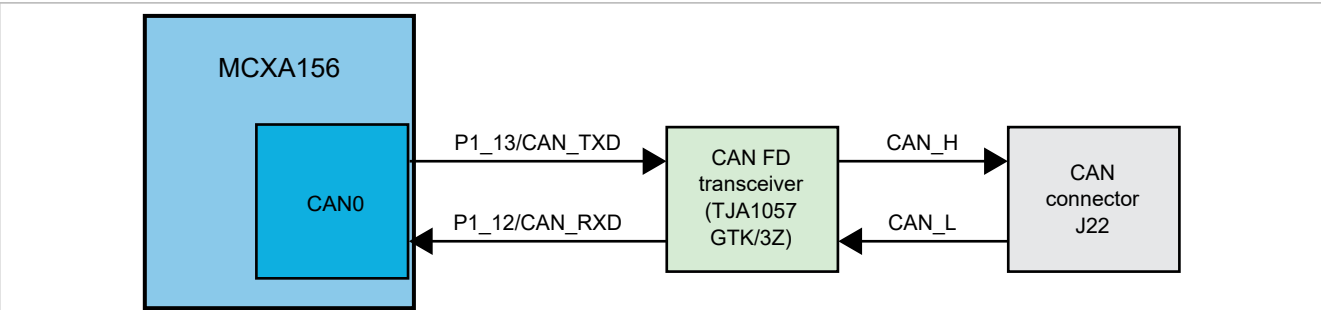
Figure 9. FlexCAN diagram
