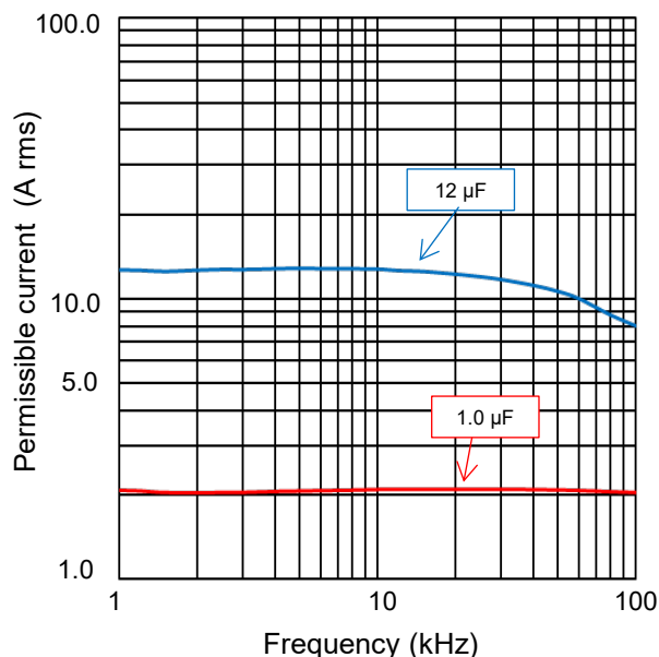
[ Permissible Current ]
