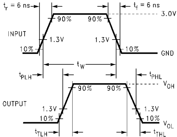
Figure 6. AC Waveforms
