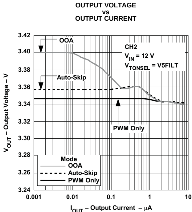
Figure 10. 3.3-V Load Regulation
