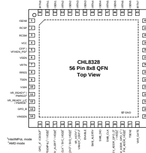
Figure 2: IR3538/CHL8328 Package Top View
