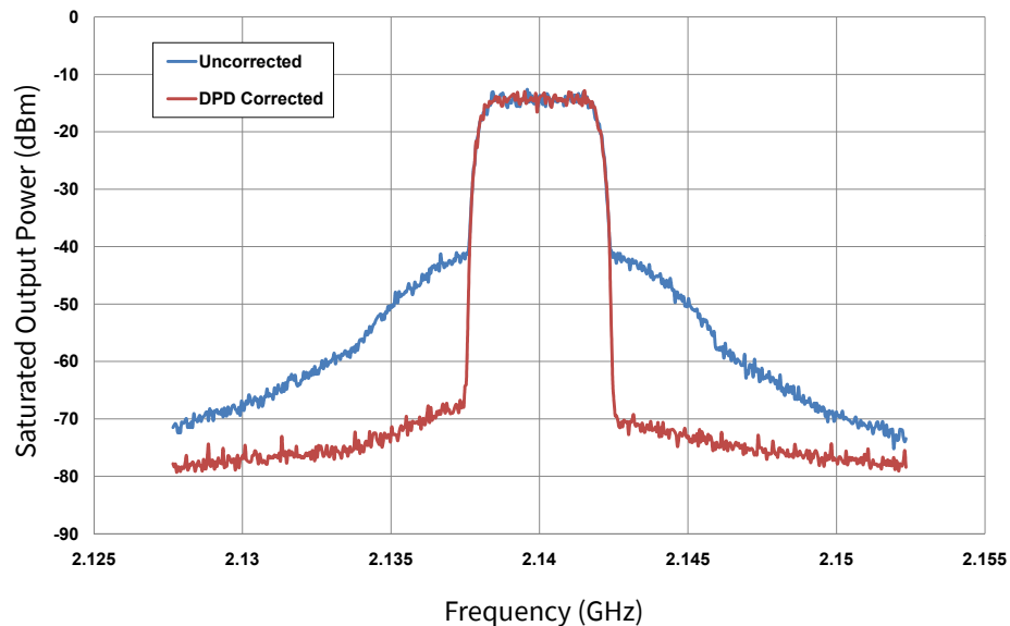
Figure 6. WCDMA Linearity with DPD Linearizer measured in CGH21120F-AMP Amplifier Circuit Single Channel WCDMA 6.5 dB PAR with CFR V_{DS} = 28\text{ V} , I_{DS} = 0.5\text{ A} , P_{OUT} = 44\text{ dBm} , Efficiency = 40%
