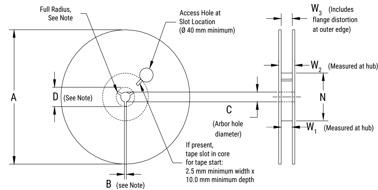
Figure 5 – Reel Dimensions
