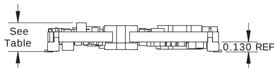
ULE 'M' TYPE SMT (GULL WING) SERIES MAXIMUM HEIGHTS
