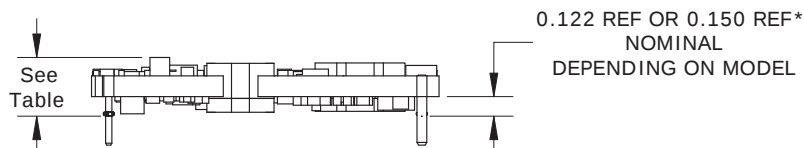
ULE THRU-HOLE SERIES MAXIMUM HEIGHTS
