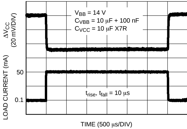
Figure 7. Load Transient Response ( I_{CC} 100 \mu\text{A} to 50 mA)
