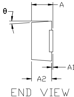
SOD-123-2 1.65x2.70x0.90 CASE 498 ISSUE E
