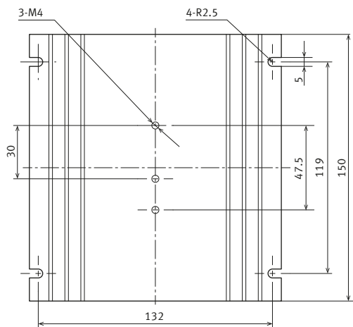
External dimensions
