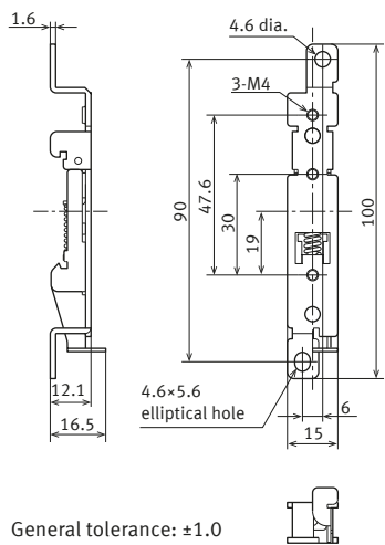
External dimensions
