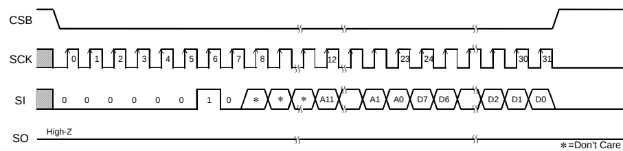
Figure 38. Write command
