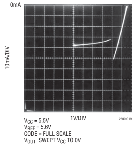
Short-Circuit Output Current vs V_{OUT} (Sourcing)
