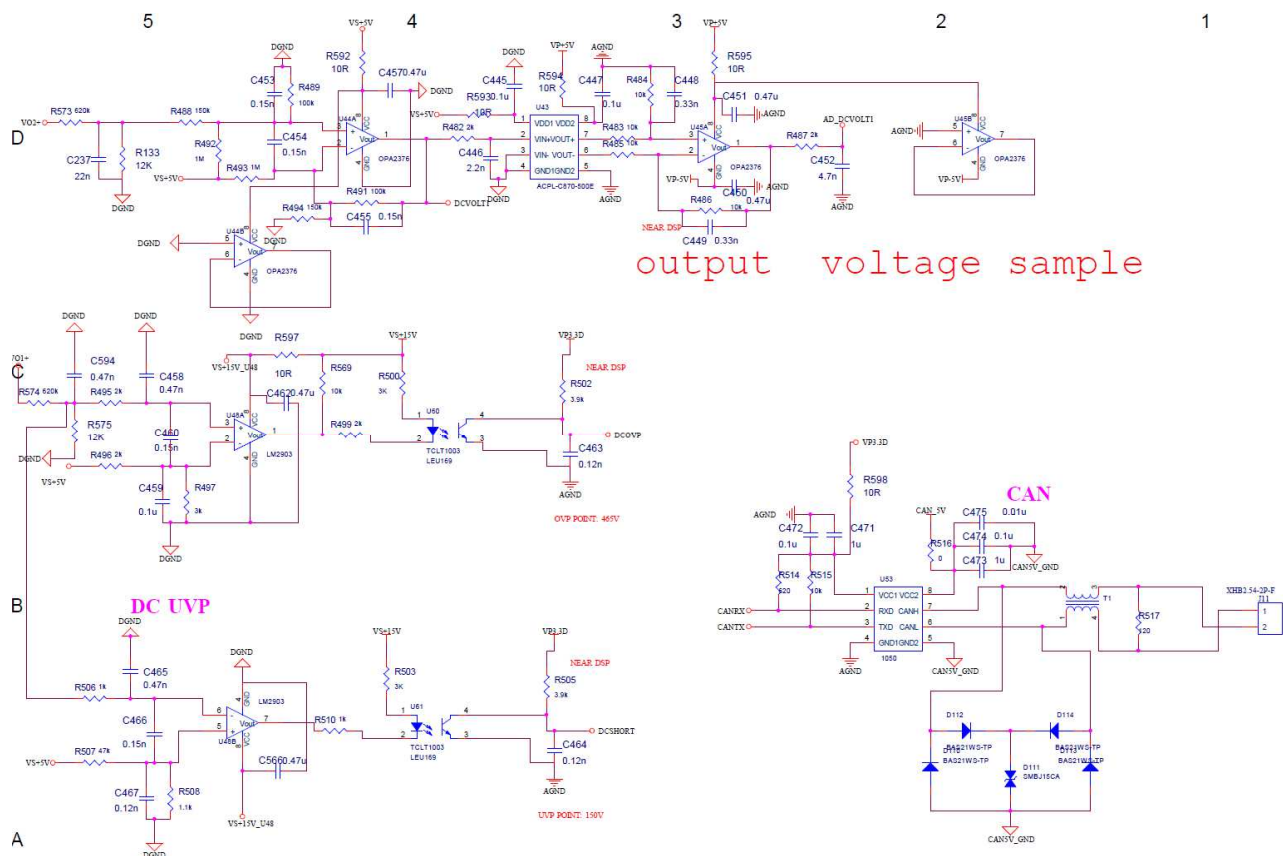
Figure 4 c: Schematic of Control Board: Output Voltage Sample and CAN Interface
