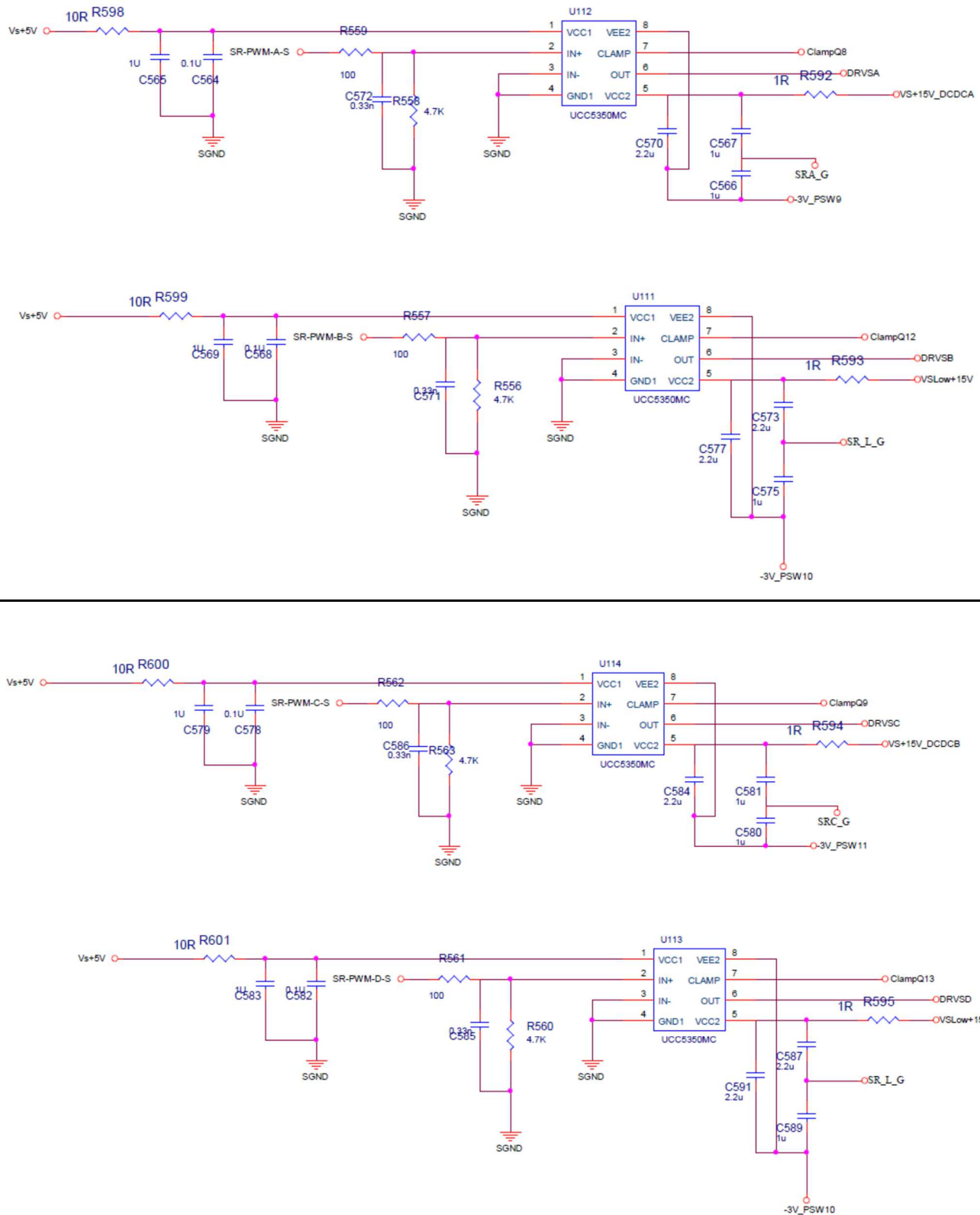
Figure 3 q: Schematic of Power Board: DC/DC Battery-Side Drives.
