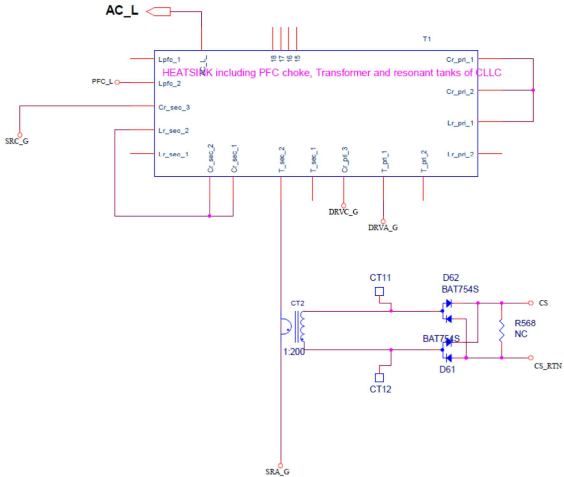
Figure 3 d: Schematic of Power Board: DC/DC Main Power.
