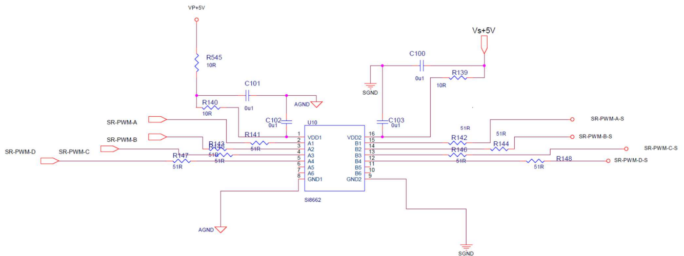
Figure 3 e: Schematic of Power Board: Signal Isolation.
