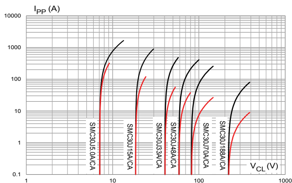
Figure 5. Maximum peak pulse current versus clamping voltage
