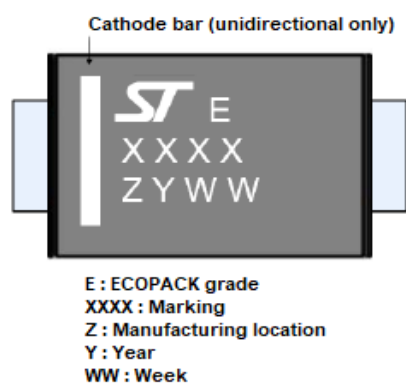
Figure 15. Marking layout
