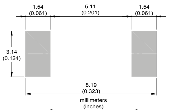
Figure 14. Footprint recommendation
