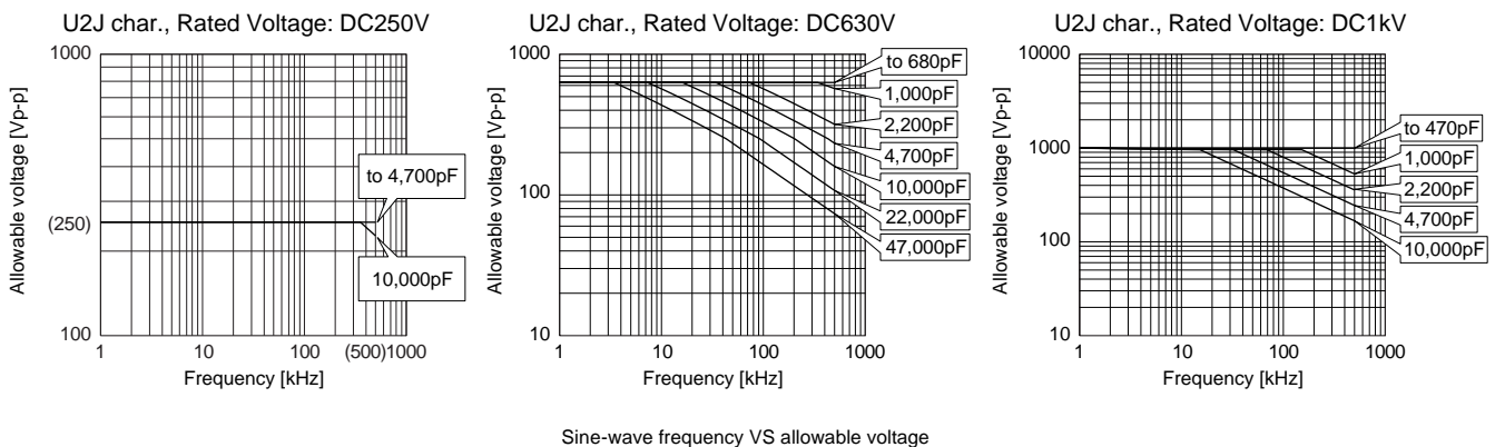
Sine-wave frequency VS allowable voltage
