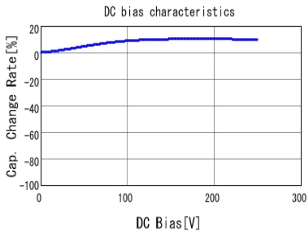
■ DE1E3KX332MA4BN01F C-DC bias capchange, 20.0degC, AC1
