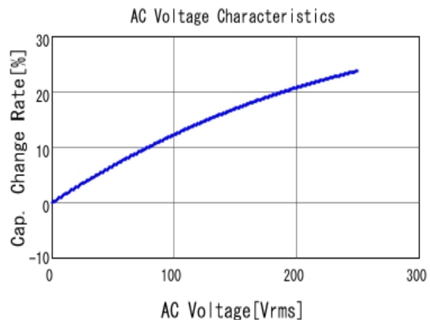
■ DE1E3KX332MA4BN01F C-AC Voltage capchange, DC0V, 20.0
