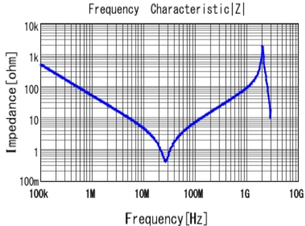
■ DE1E3KX332MA4BN01F |Z| DC0V, 20degC
