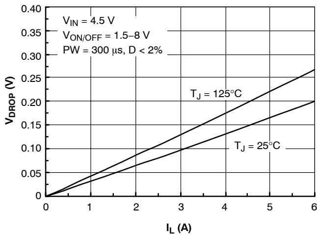
Figure 6. Conduction Voltage Drop Variation with Load Current
