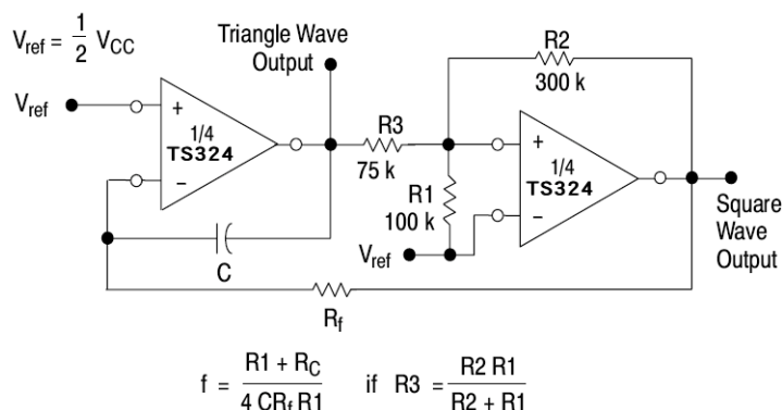
Figure 12. Function Generator
