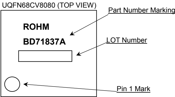
Figure 9-1. Marking Diagram
