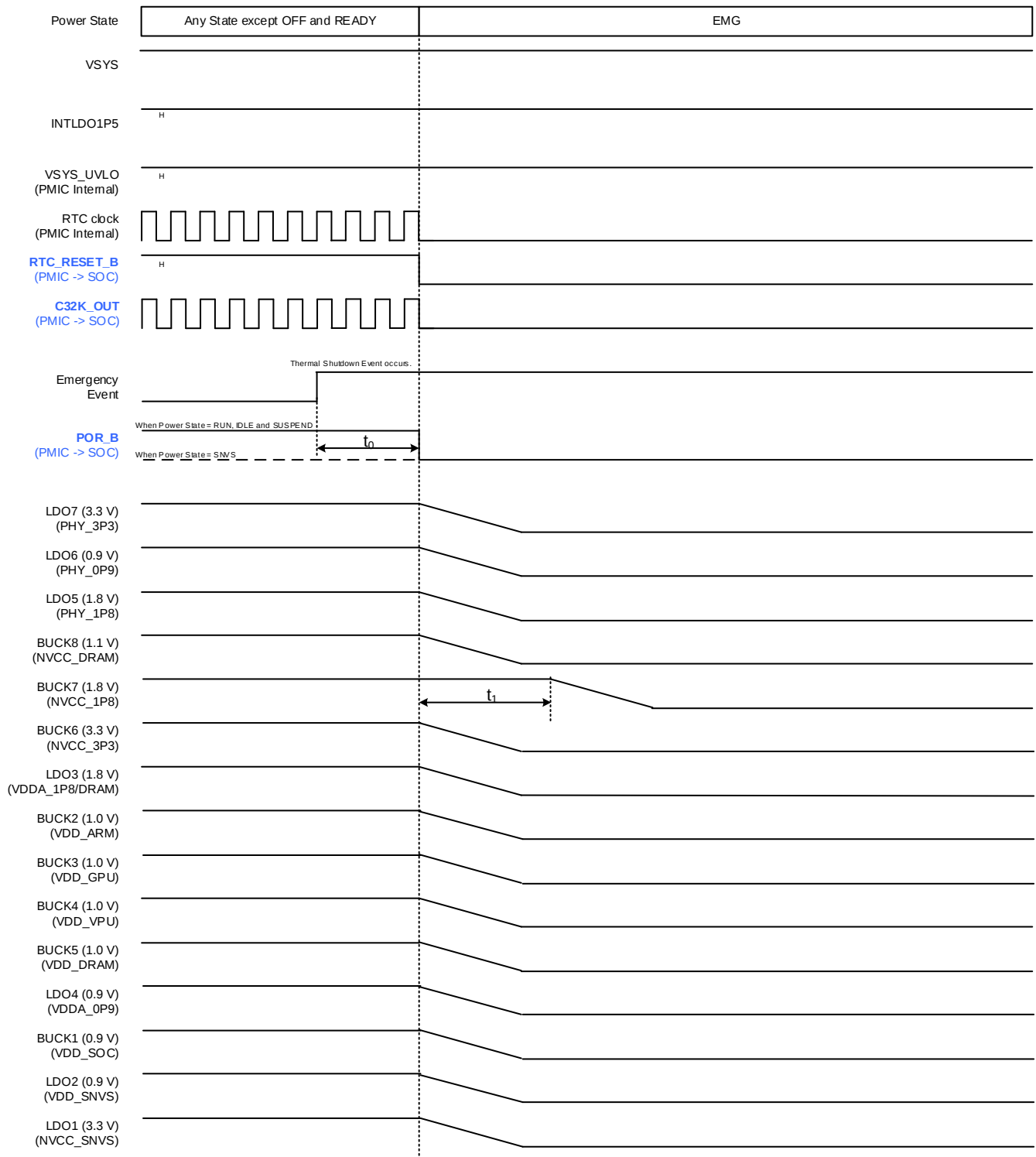
Figure 3-29. Emergency Shutdown
