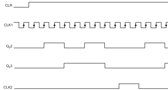
Figure 2. Timing Diagram
