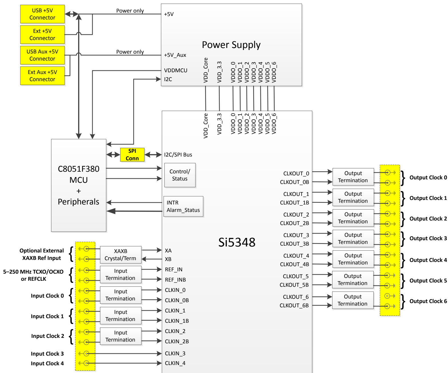
Figure 1.1. Si5348-E-EVB Functional Block Diagram
