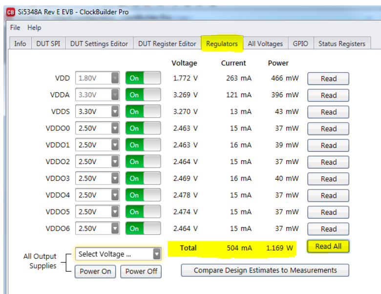
Figure 6.9. EVB GUI Window
