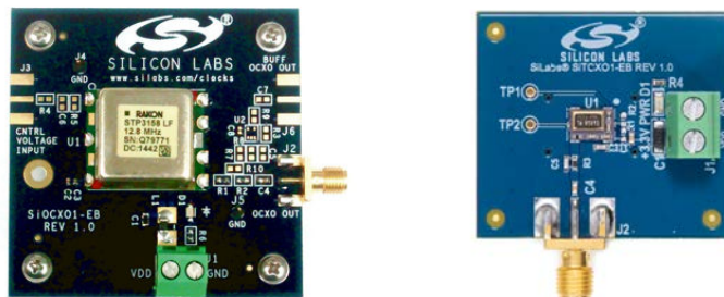
Figure .2. SiOCXO1-EB (left) SiTCXO1-EB (right)
