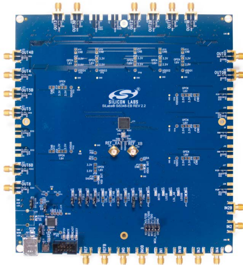
Figure .1. Si5348-EVB
