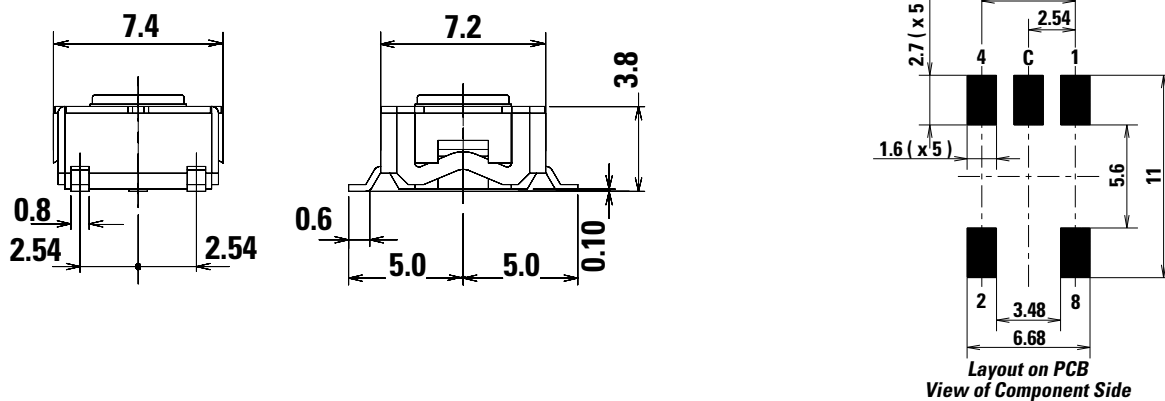
G - Surface Mount (mm)
