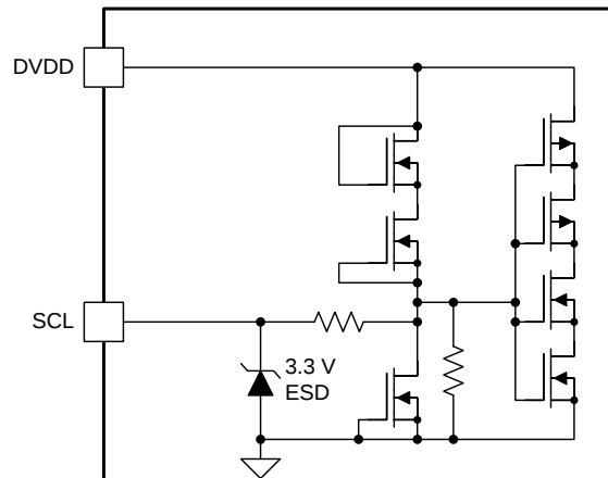
Figure 10. SCL Pin
