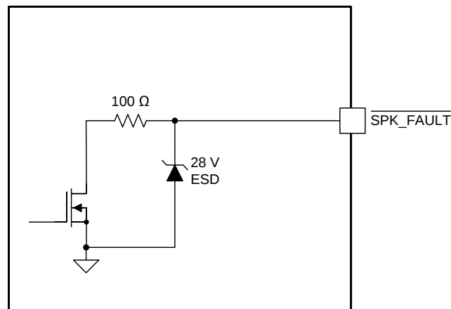
Figure 17. SPK_FAULT Pin
