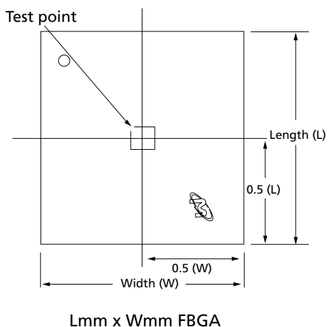
Figure 12: Example Temperature Test Point Location
