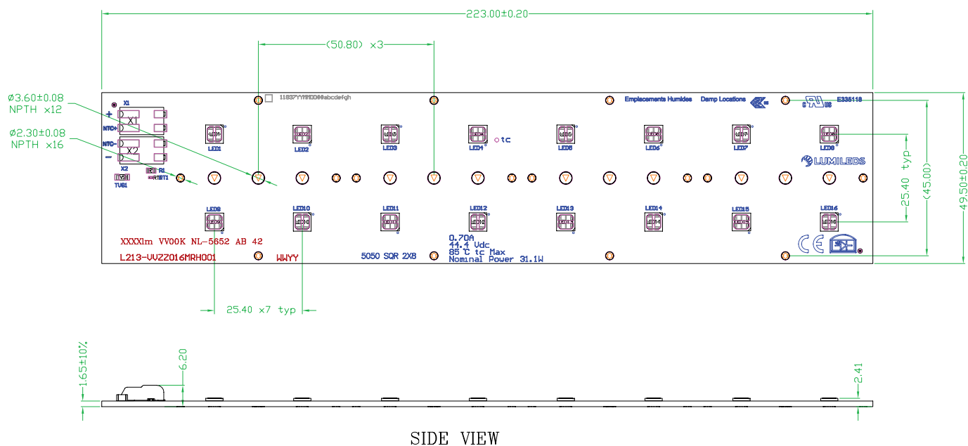
Figure 10. Mechanical dimensions for L213-xxxx016MRH001.
