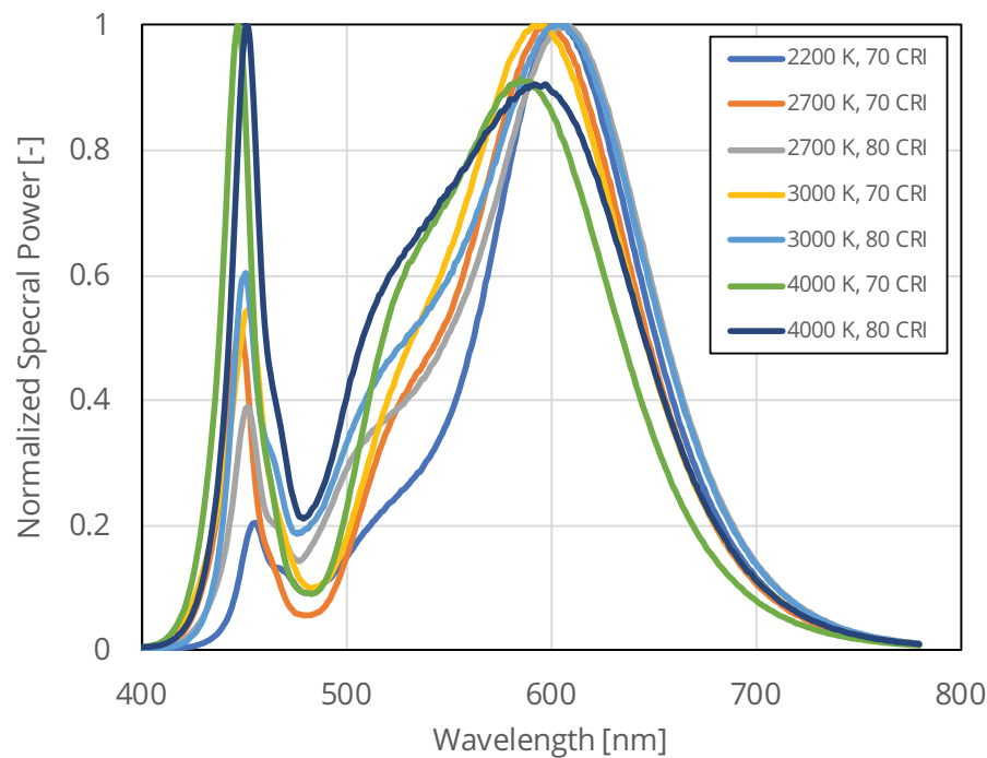
Figure 1. Typical normalized spectral power vs. wavelength for LUXEON XR-5050 SQR at 700mA, T c =85°C.
