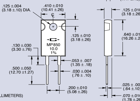
Figure 3 TO-220 Style MP850
