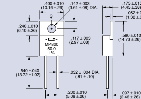
Figure 1 Metal Tab TO-220 Style MP820 and MP821
