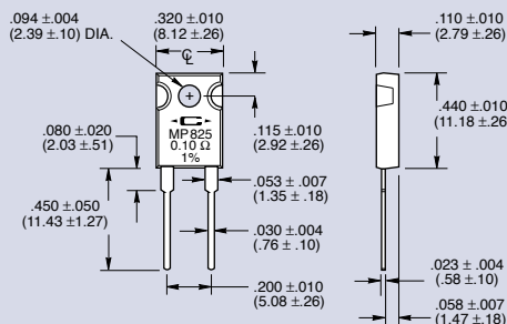
Figure 2 TO-126 Style MP825
