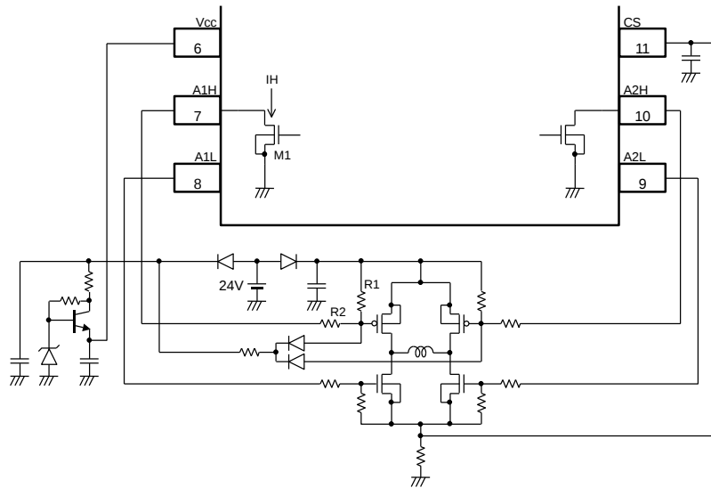
Figure 47. 24V application
