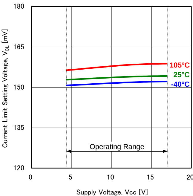
Figure 20. Current Limit Setting Voltage vs Supply Voltage
