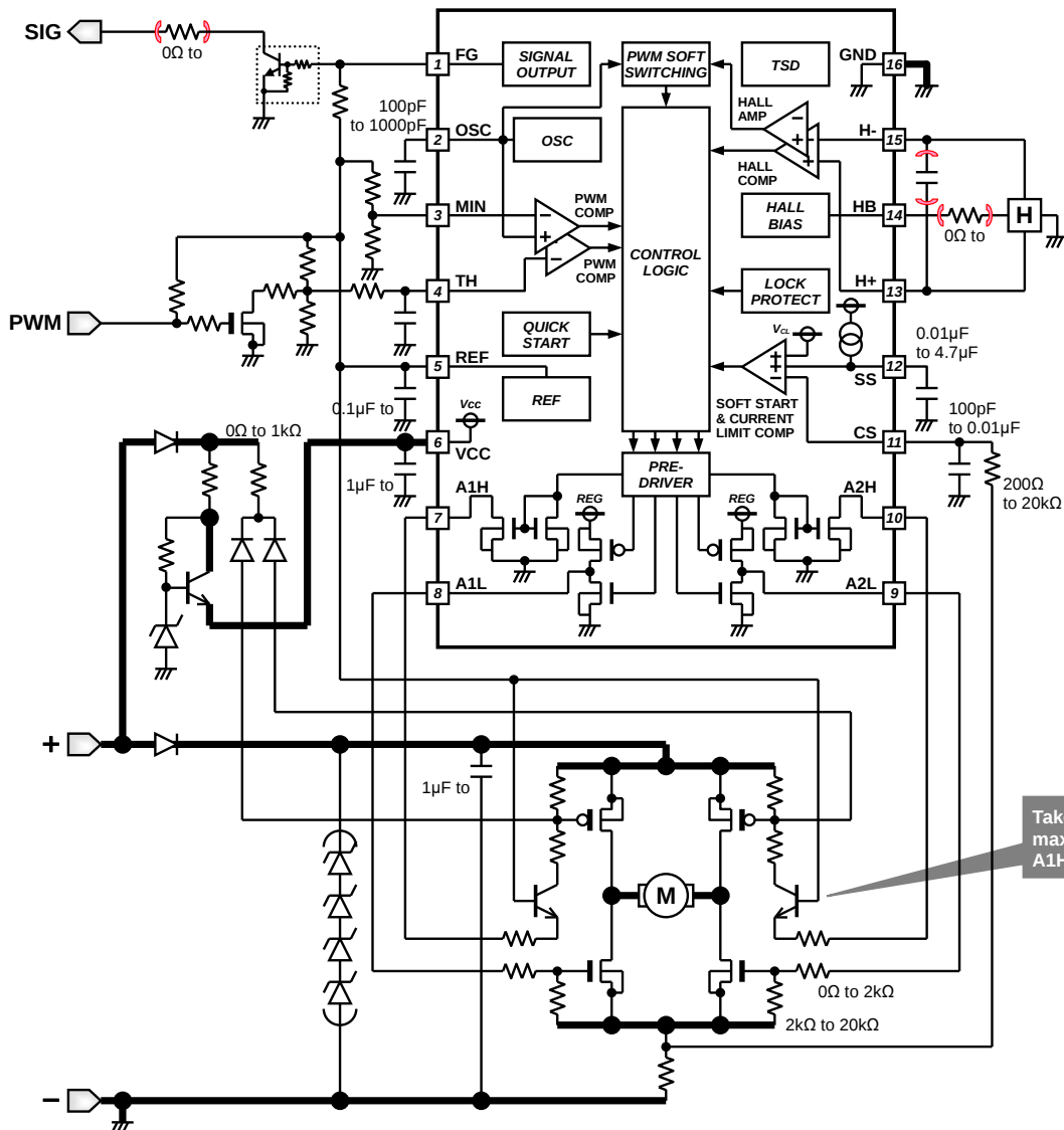
Figure 30. Over 48V power supply application of PWM input
