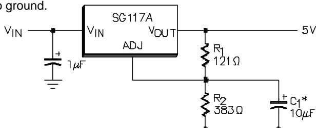
Figure 19 • Improving Ripple Rejection
