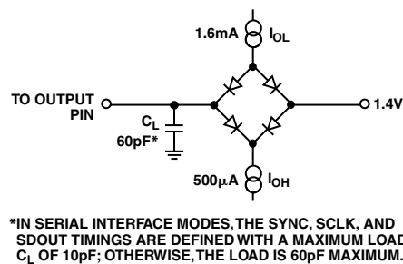
Figure 1. Load Circuit for Digital Interface Timing, SDOOUT, SYNC, SCLK Outputs, C_L = 10 \text{ pF}
