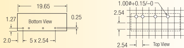
Recommended Footprint Details
