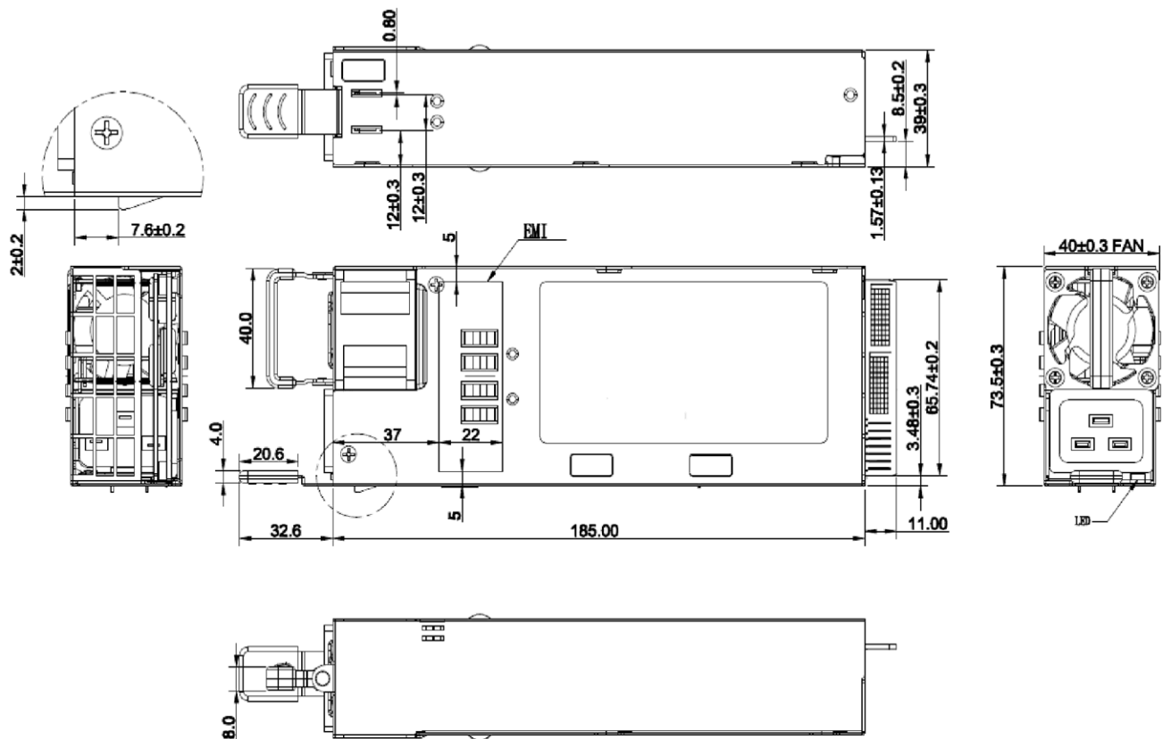
Figure 18. Mechanical Drawing
