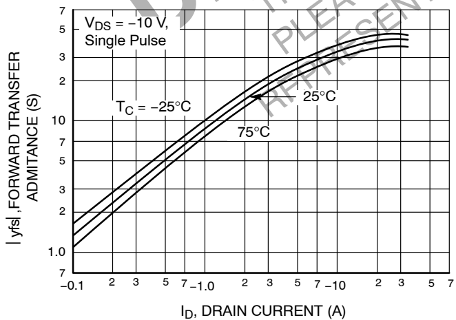
Figure 6. |y_{fs}| - I_D
