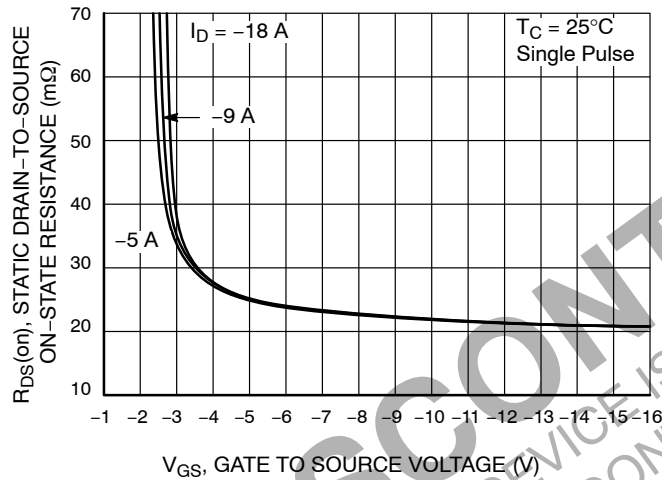
Figure 4. R_{DS(on)} - V_{GS}
