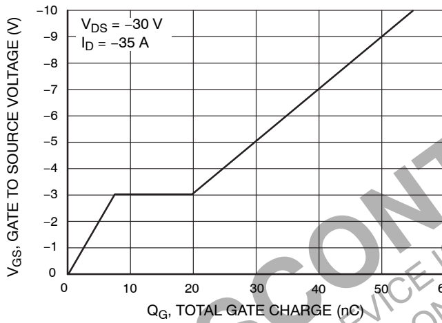
Figure 10. V_{GS} - Q_g
