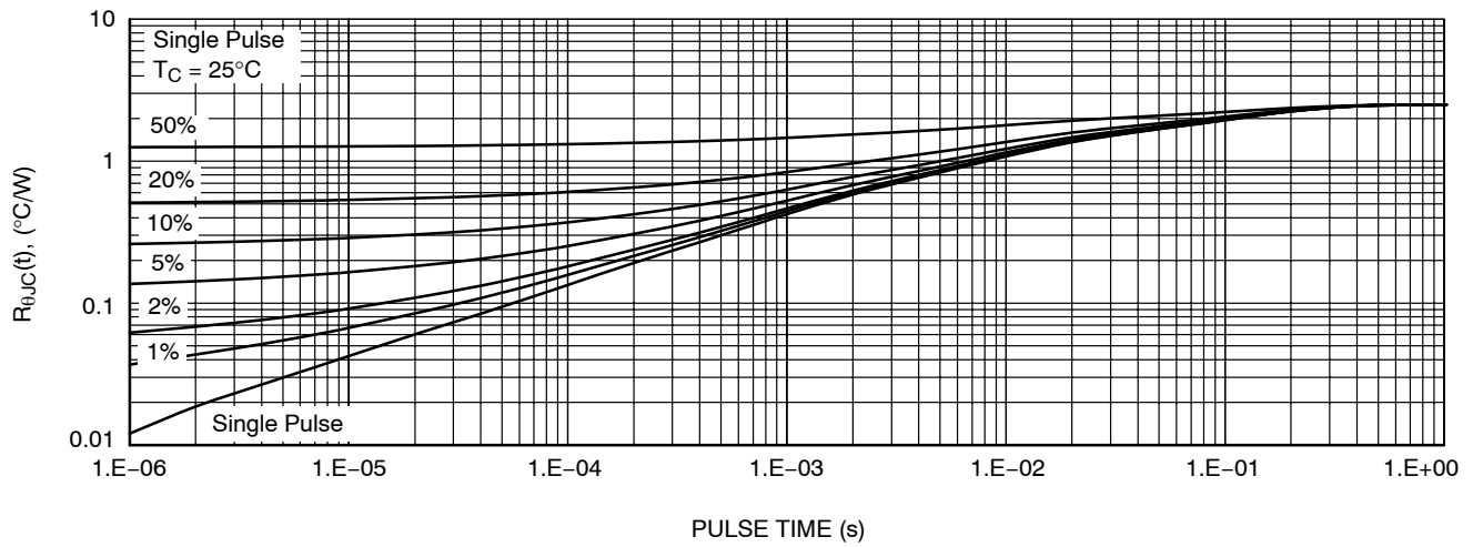
Figure 14. Thermal Response
