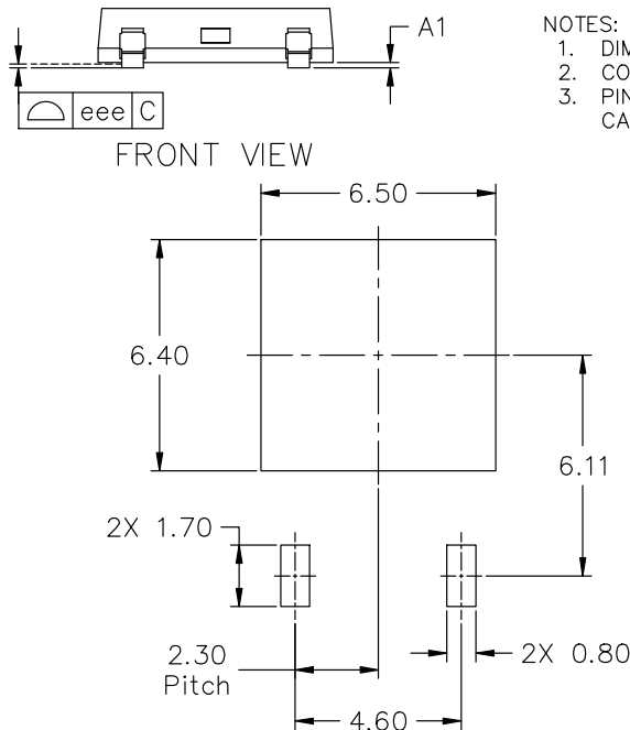
RECOMMENDED MOUNTING FOOTPRINT
