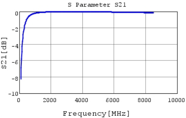
GCQ1555C1H6R7CB01 S21 DCOV, 25degC
