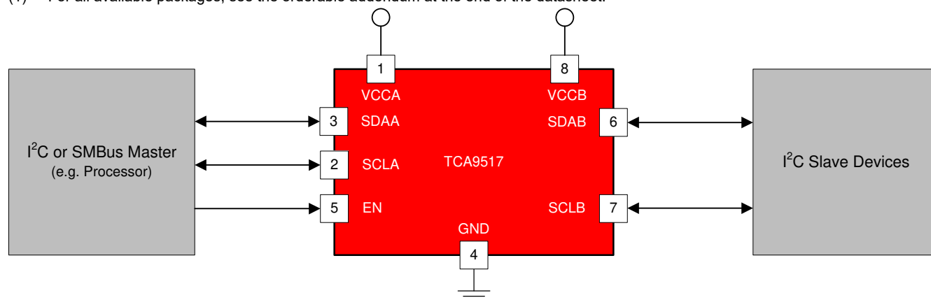
Simplified Schematic
