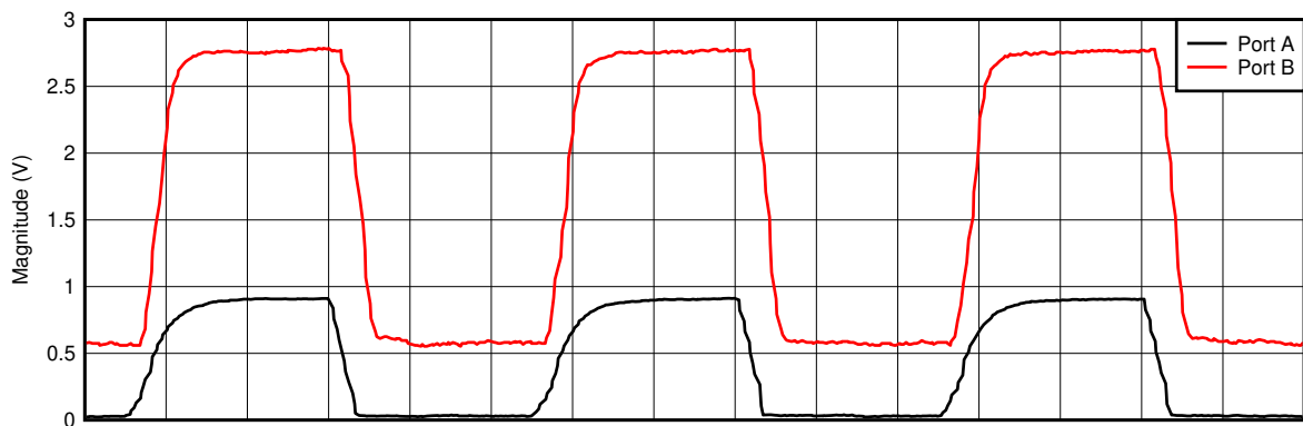
Figure 8-6. Voltage Translation at 400 kHz, V_{CCA} = 0.9\text{ V} , V_{CCB} = 2.7\text{ V}
