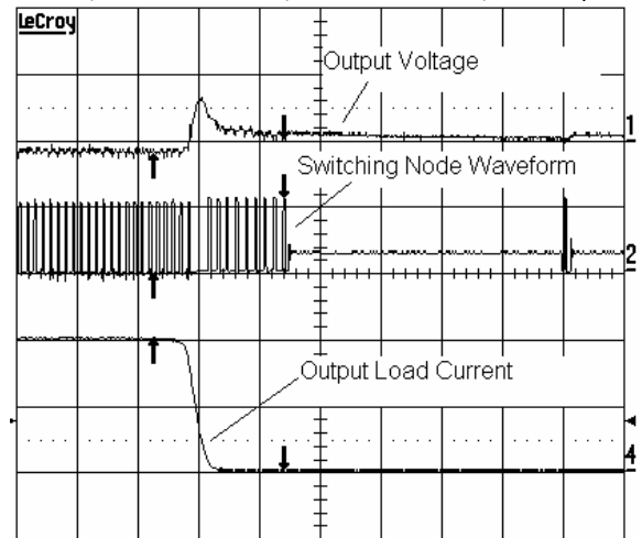
Load Transient Test ( V_{IN}=5V , V_{OUT}=1.2V , I_{OUT}=2A to 0A , PSAVE Mode Enabled, L_{OUT}=1.3\mu H , C_{OUT}=2 \times 22\mu F , Channel 1: 50mV/Div, Channel 2: 5V/Div, Channel 4: 1A/Div, Time: 10μs/Div)
