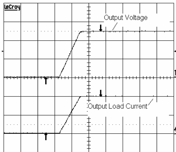
Load Transient Test ( V_{IN}=5V , V_{OUT}=1.2V , I_{OUT}=0A to 2A , Forced Continuous Conduction Mode, L_{OUT}=1.3\mu H , C_{OUT}=2 \times 22\mu F , Channel 1: 50mV/Div, Channel 2: 5V/Div, Channel 4: 1A/Div, Time: 10 \mu s /Div)
