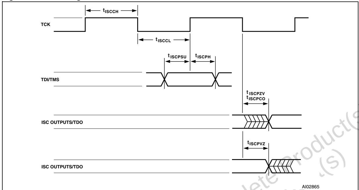
Figure 45. ISC Timing
