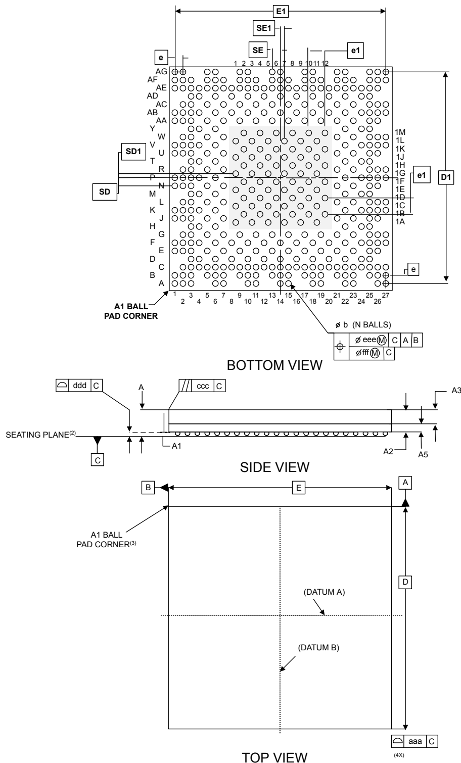
Figure 66. VFBGA424 - Outline
