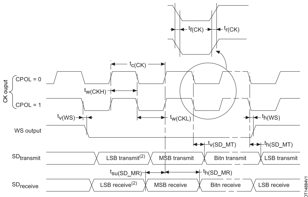
Figure 51. I2S master timing diagram (Philips protocol)
