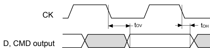
Figure 56. SDRAM DDR mode
