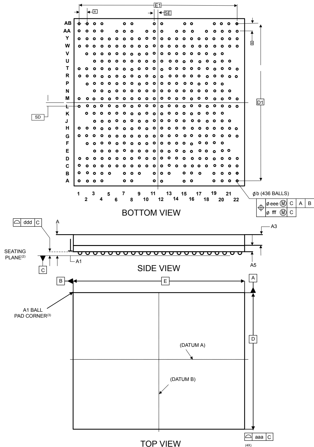
Figure 67. TFBGA436 - Outline
