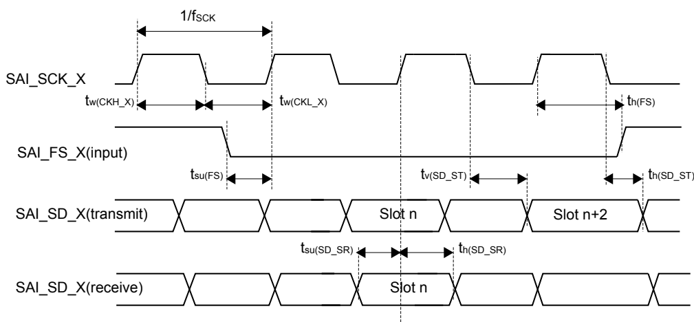
Figure 53. SAI slave timing waveforms
