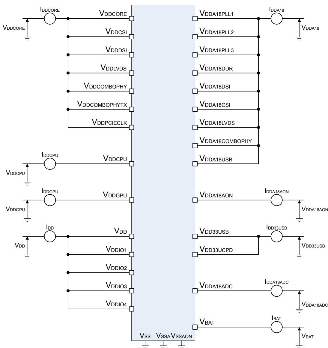
Figure 12. Current consumption measurement scheme
