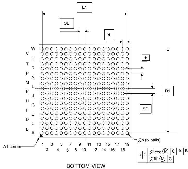
Figure 65. VFBGA361 - Outline
