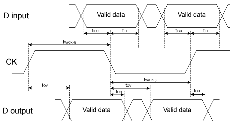
Figure 56. SDRAM DDR mode
