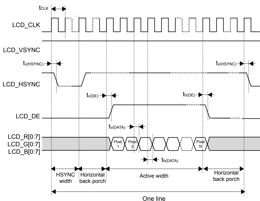
Figure 45. LCD-TFT horizontal timing diagram
