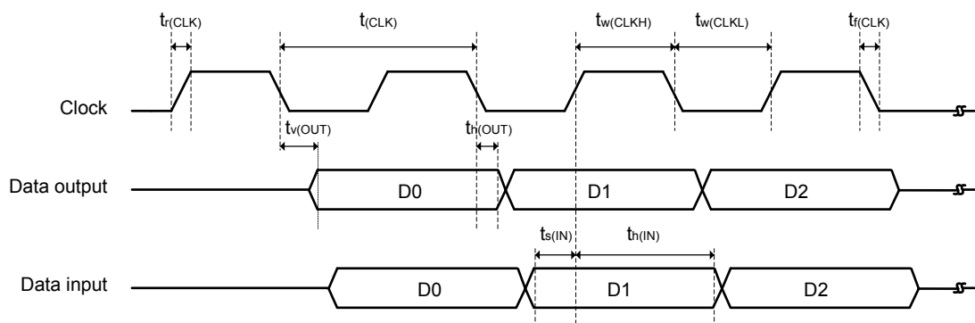
Figure 31. OCTOSPI timing diagram - SDR mode
