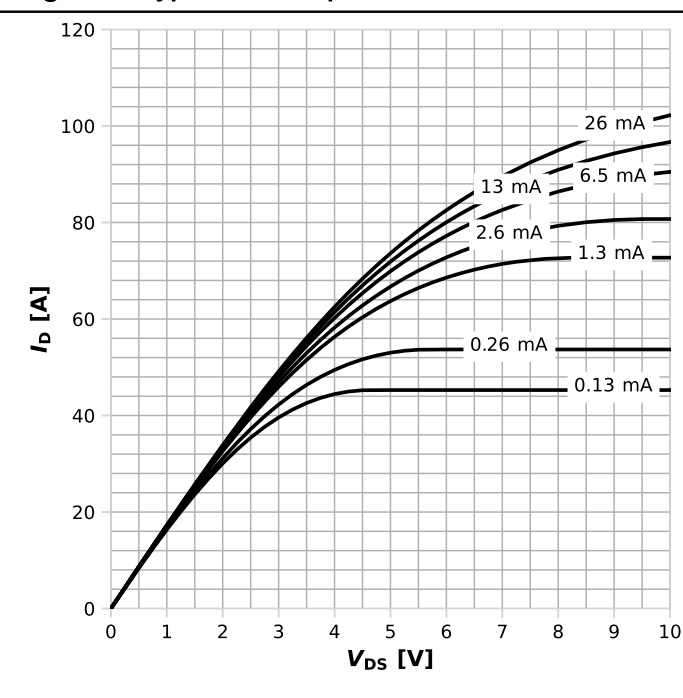
Diagram 7: Typ. static* output characteristics
