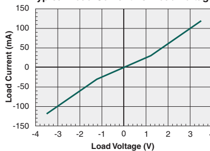
Typical Load Current vs. Load Voltage
