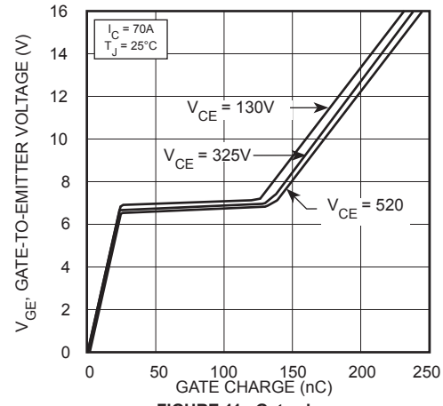
FIGURE 11, Gate charge
