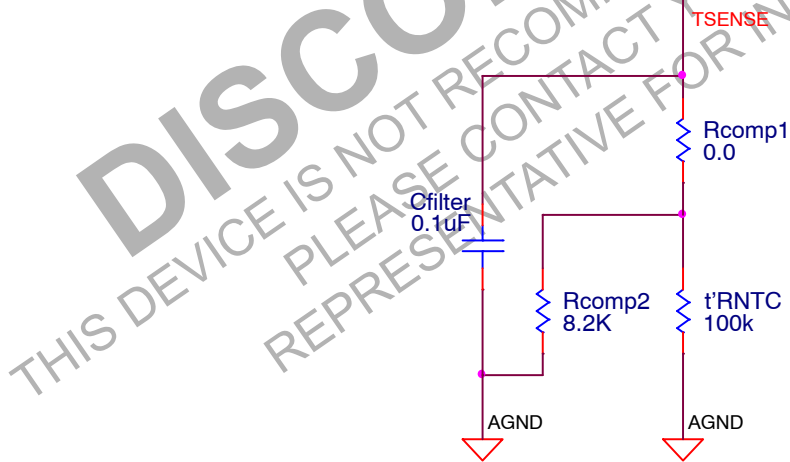
Figure 8. TSENSE Circuit
