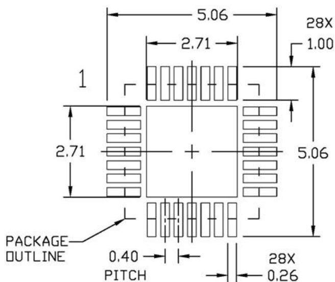
Figure 17. Alternative Extended Soldering Footprint
