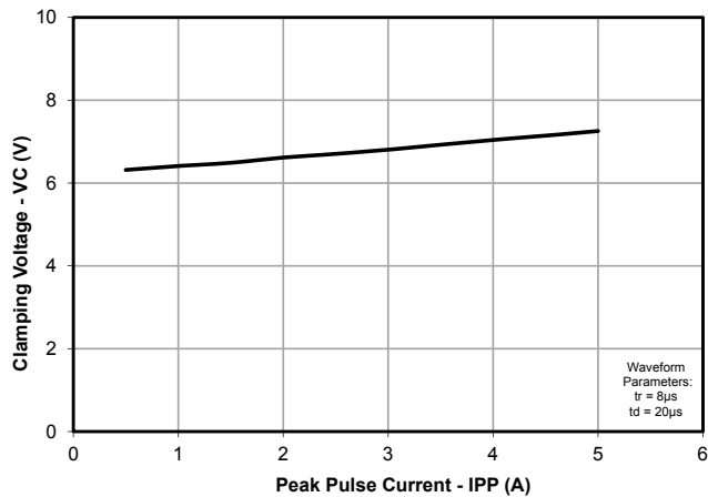
Clamping Characteristic (8/20us Waveform)
