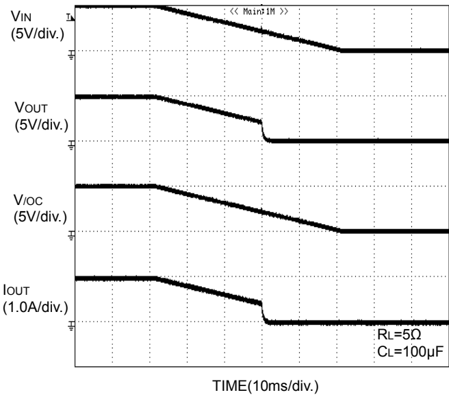
Figure 39. UVLO Response when Decreasing V_{IN}
