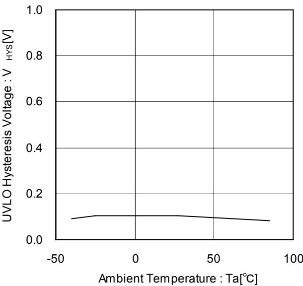
Figure 19. UVLO Hysteresis Voltage vs Ambient Temperature
