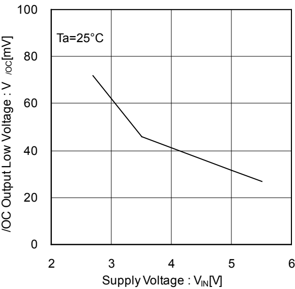
Figure 16. /OC Output Low Voltage vs Supply Voltage
