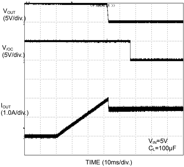
Figure 33. Over-Current Response Ramped Load
