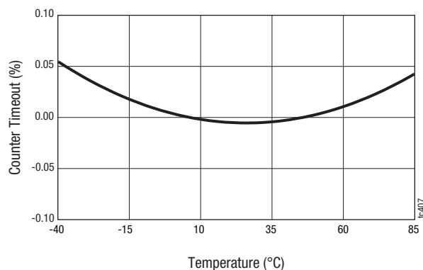
Figure 19. Counter Timeout vs Temperature ( C_{CT} = 0.1 μF)
